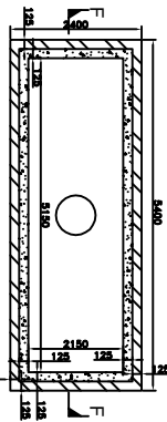
DEL. OF UNDER GROUND WATER RESERVOIR
